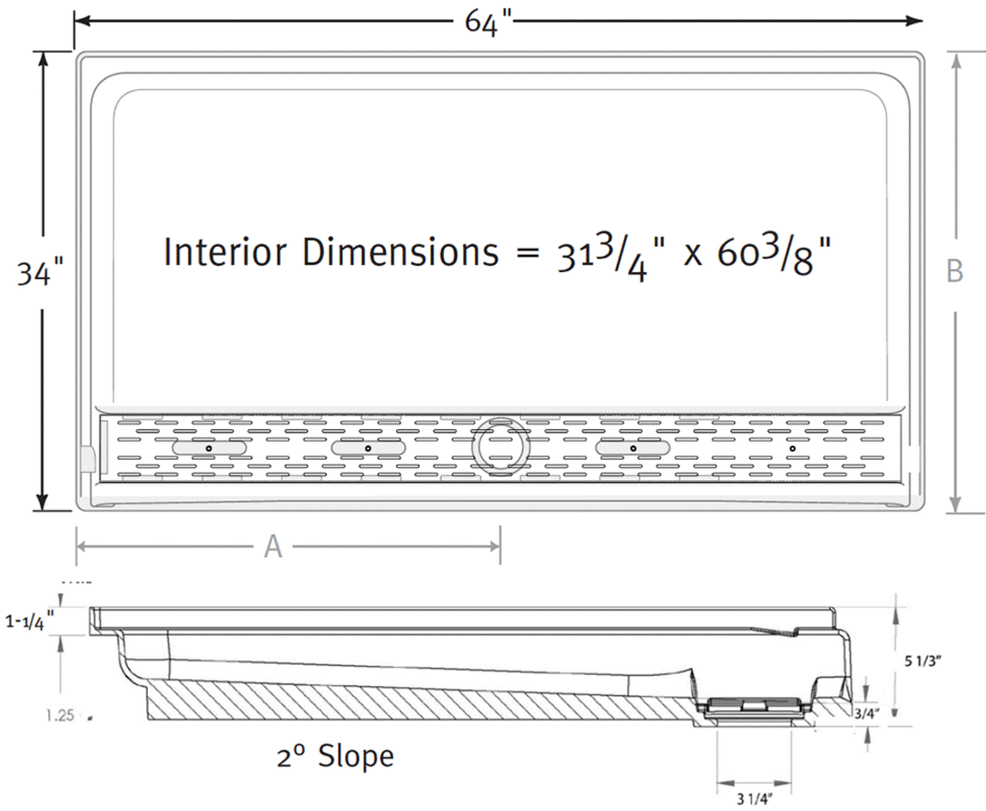
Trough system drains into standard 2" drain pipe.
